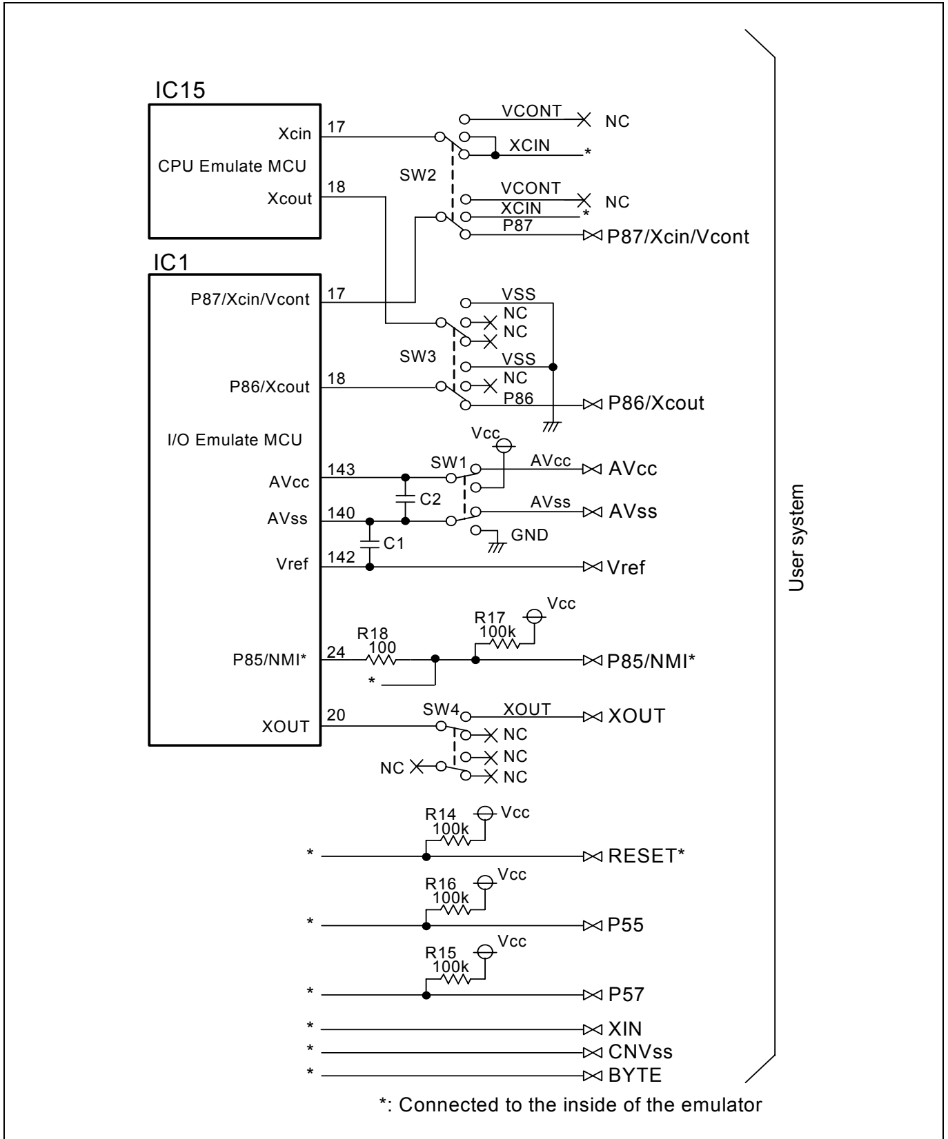
Figure 4.1 Connection diagram (1/2)
